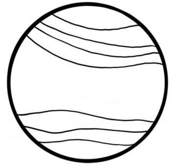
Neptune
