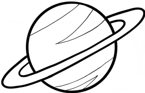
Saturn
