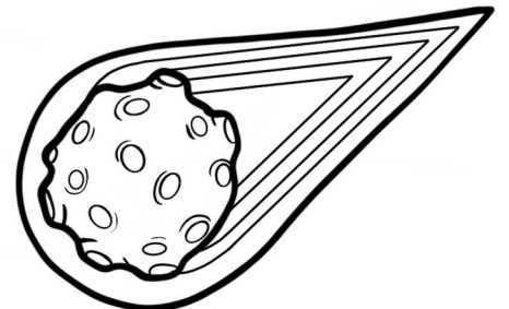
Comet
