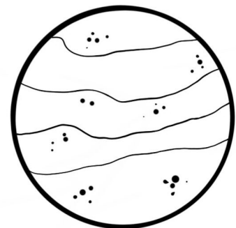
NEPTUNE
